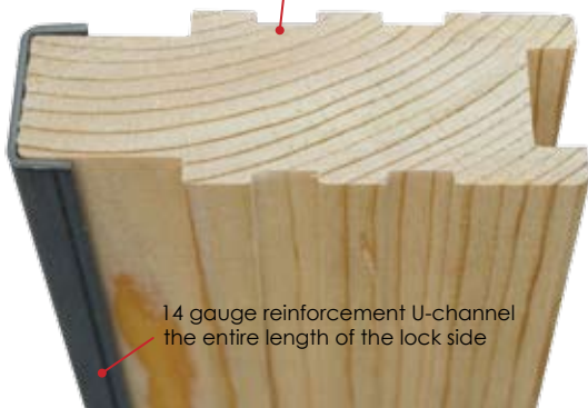
4 1/4" Finger joint lock block the entire length of the lock side
