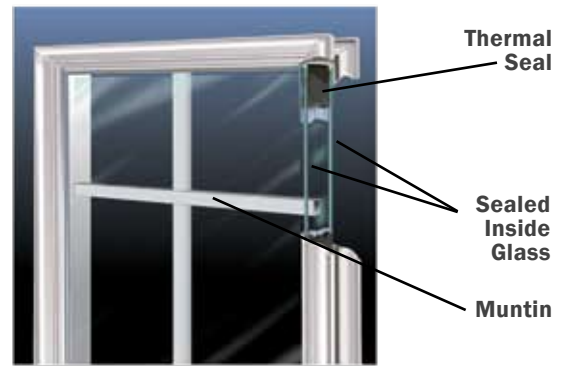
Internal Muntin Design
